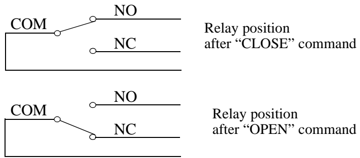
Figure 4-4. Write a "1" or "0" to the Register Bit to Close/Open the Relay
