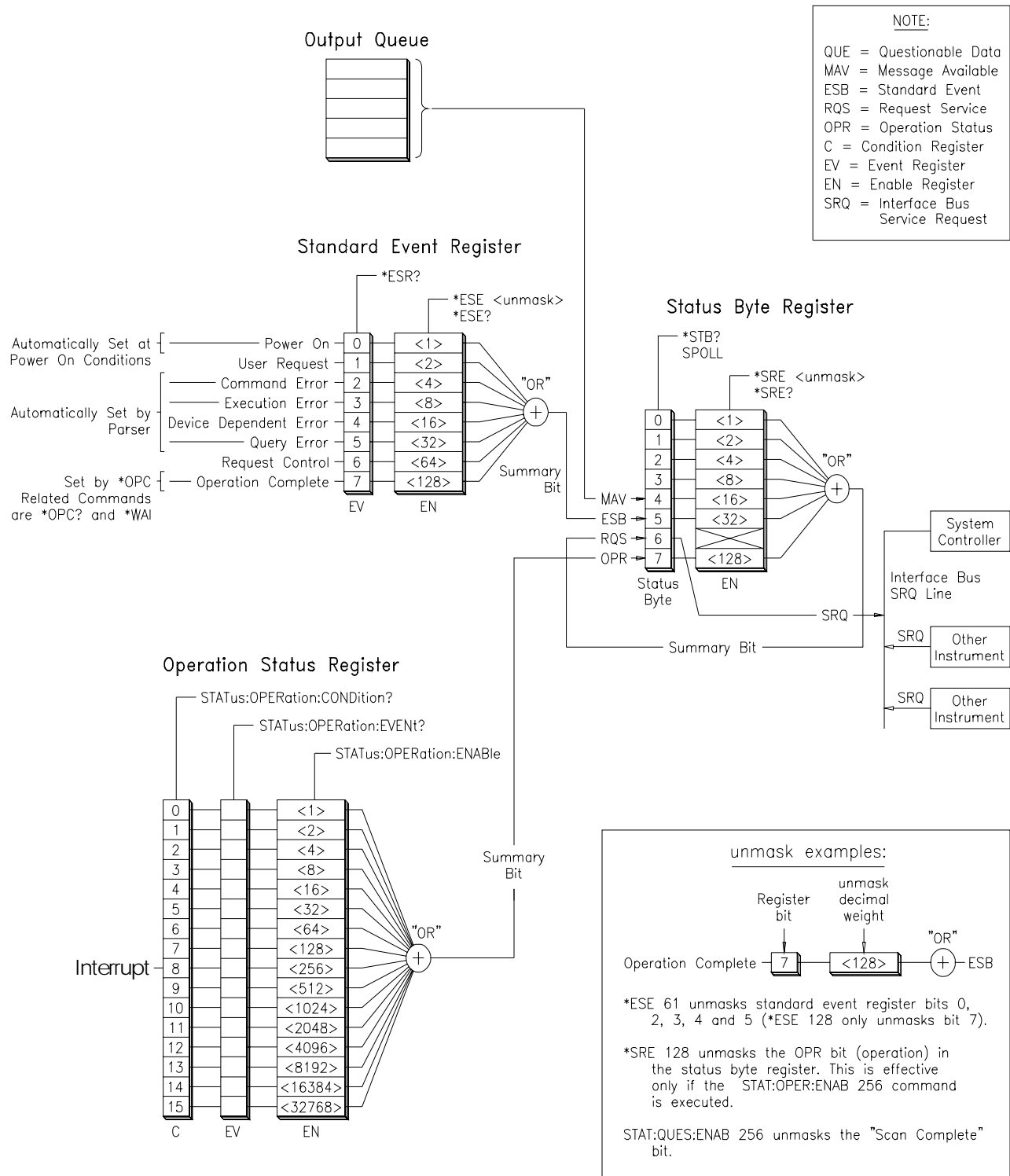
Figure 3-2. Status System
